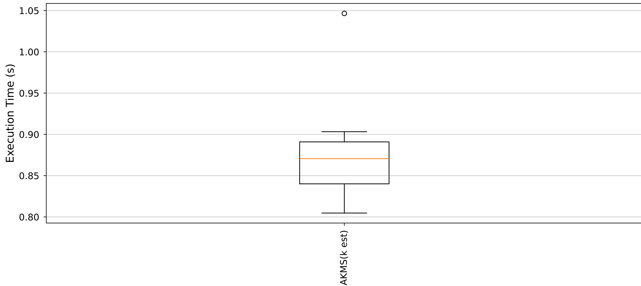
YARA Rules Execution Time Distribution (Cluster34_Size5 dataset)
